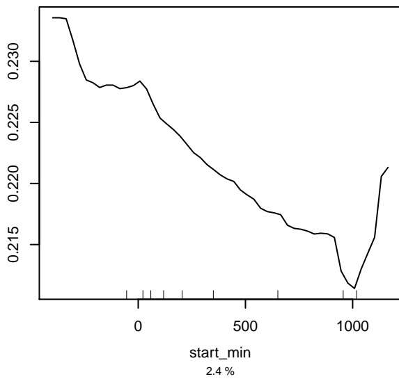
Partial dependence on start_min
