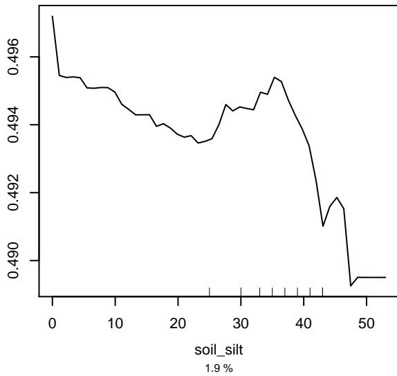
Partial dependence on soil_silt
