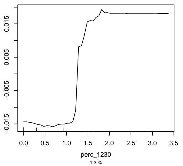
Partial dependence on perc_1230
