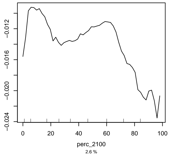
Partial dependence on perc_2100
