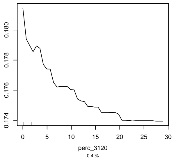
Partial dependence on perc_3120
