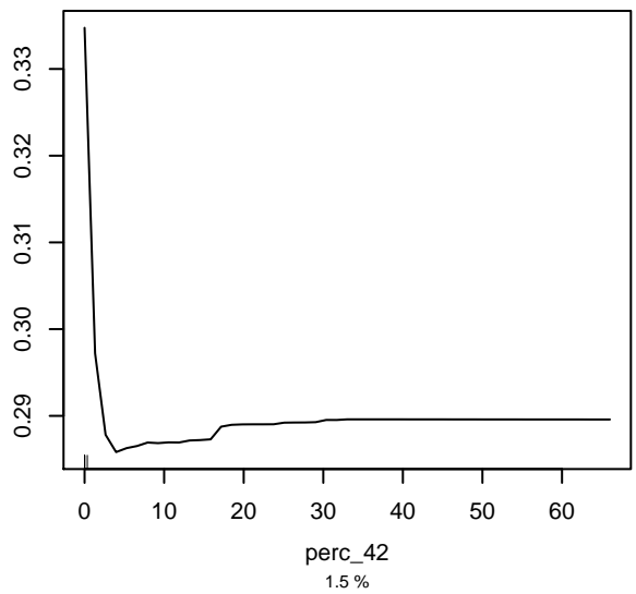
Partial dependence on perc_42
