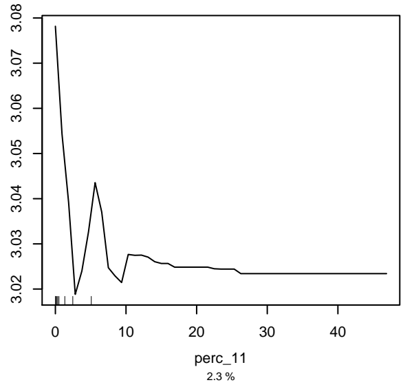
Partial dependence on perc_11
