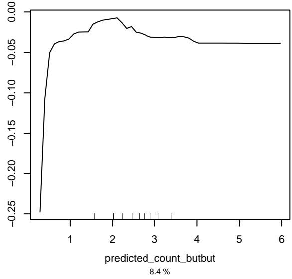
Partial dependence on predicted_count_butbut
