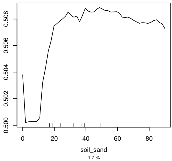
Partial dependence on soil_sand
