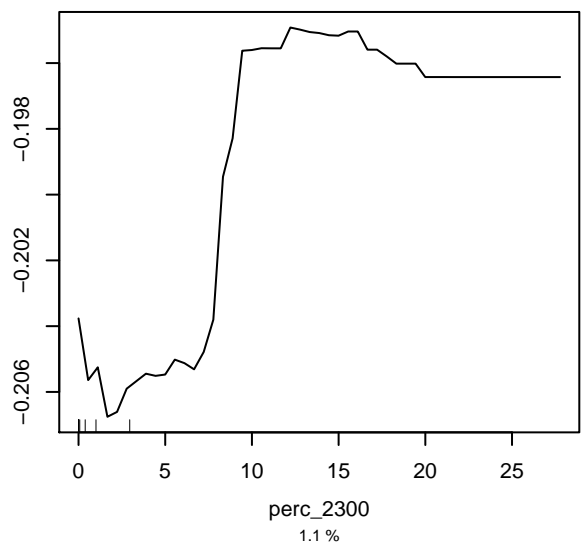
Partial dependence on perc_2300
