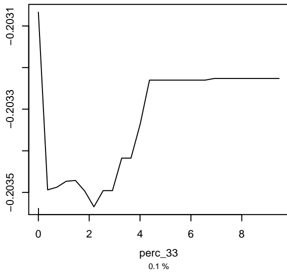
Partial dependence on perc_33
