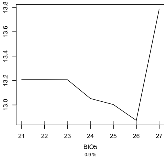
Partial dependence on BIO5
