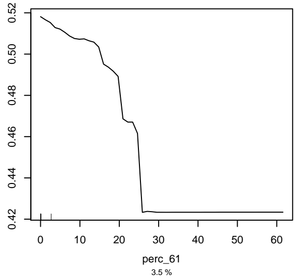
Partial dependence on perc_61
