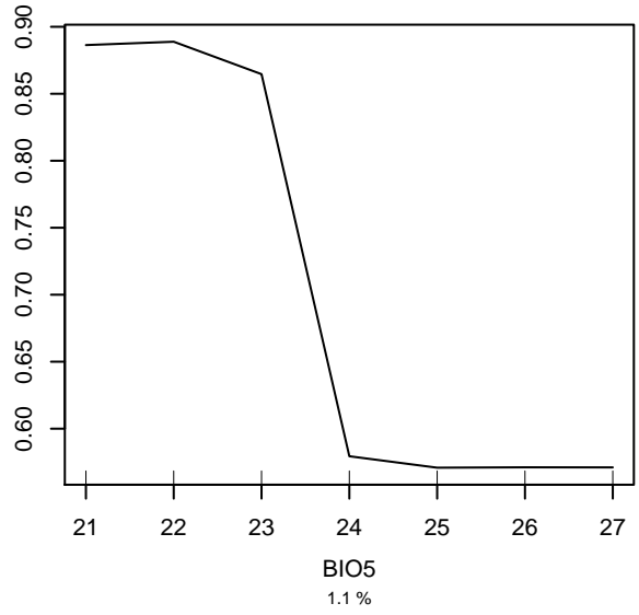
Partial dependence on BIO5
