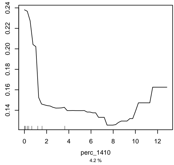
Partial dependence on perc_1410
