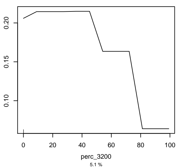
Partial dependence on perc_3200
