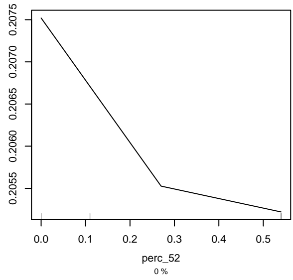
Partial dependence on perc_52
