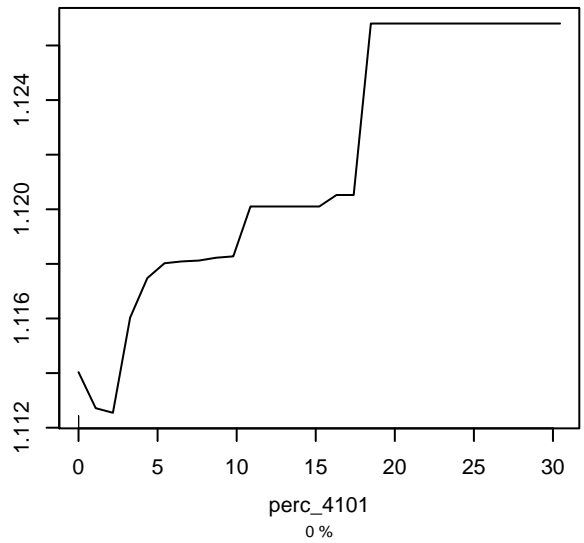
Partial dependence on perc_4101
