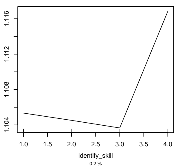
Partial dependence on identify_skill
