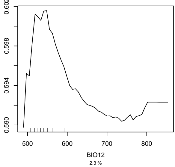
Partial dependence on BIO12
