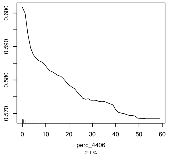
Partial dependence on perc_4406
