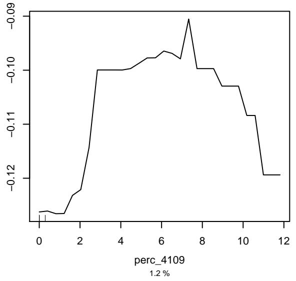
Partial dependence on perc_4109
