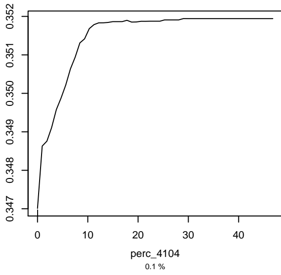
Partial dependence on perc_4104
