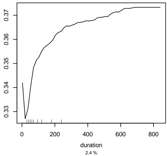
Partial dependence on duration
