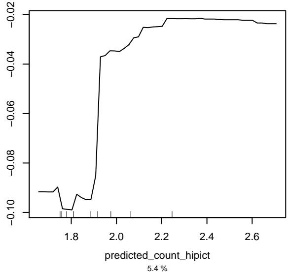
Partial dependence on predicted_count_hipict
