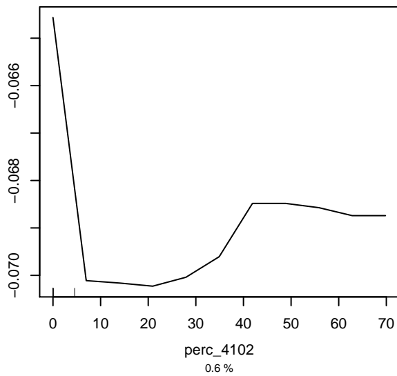
Partial dependence on perc_4102
