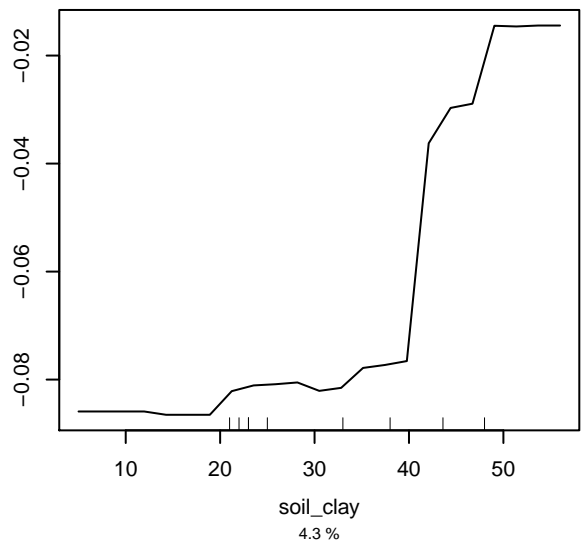
Partial dependence on soil_clay
