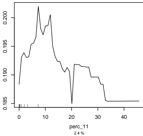
Partial dependence on perc_11
