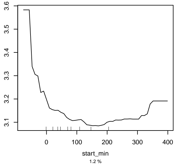
Partial dependence on start_min
