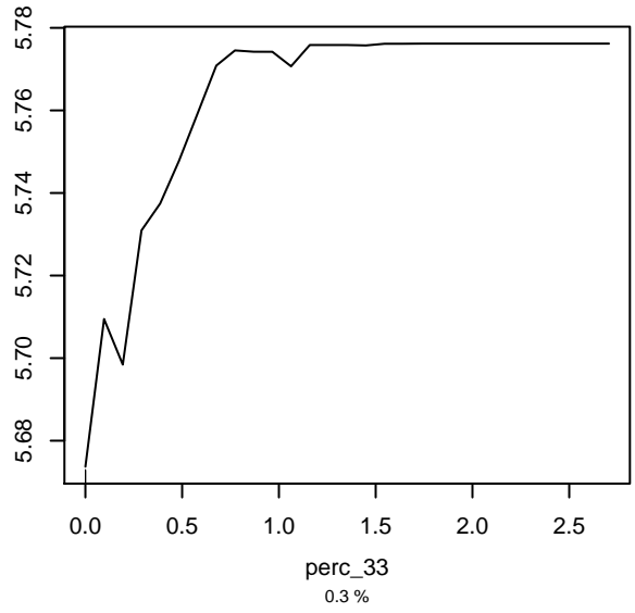
Partial dependence on perc_33
