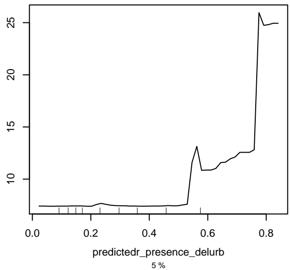
Partial dependence on predictedr_presence_delurb
