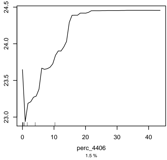
Partial dependence on perc_4406
