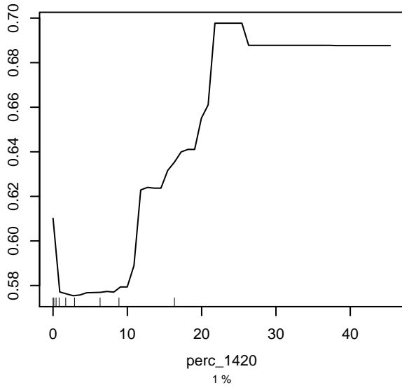
Partial dependence on perc_1420
