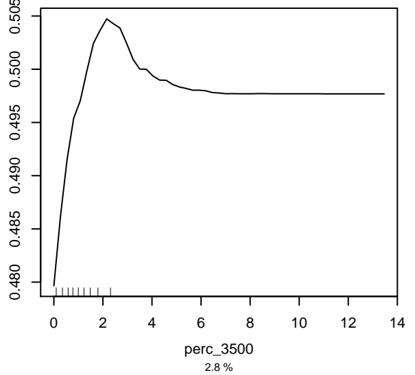
Partial dependence on perc_3500
