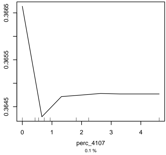
Partial dependence on perc_4107
