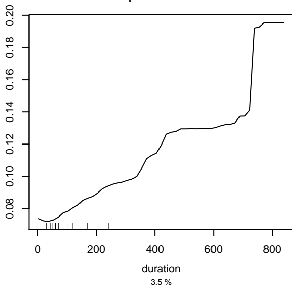
Partial dependence on duration
