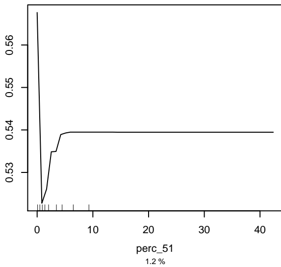
Partial dependence on perc_51
