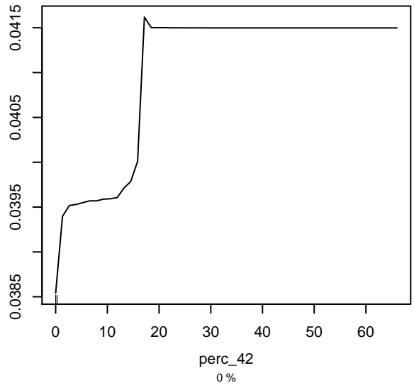
Partial dependence on perc_42
