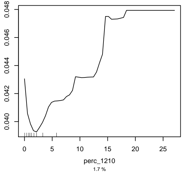
Partial dependence on perc_1210
