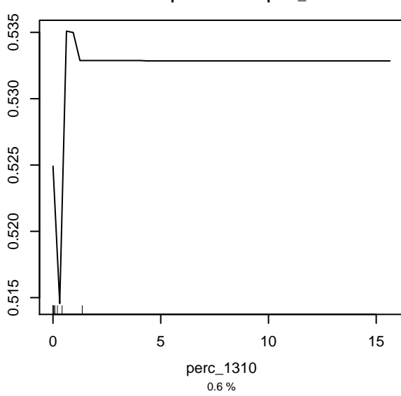
Partial dependence on perc_1310
