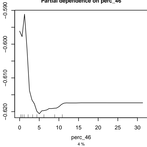
Partial dependence on perc_46
