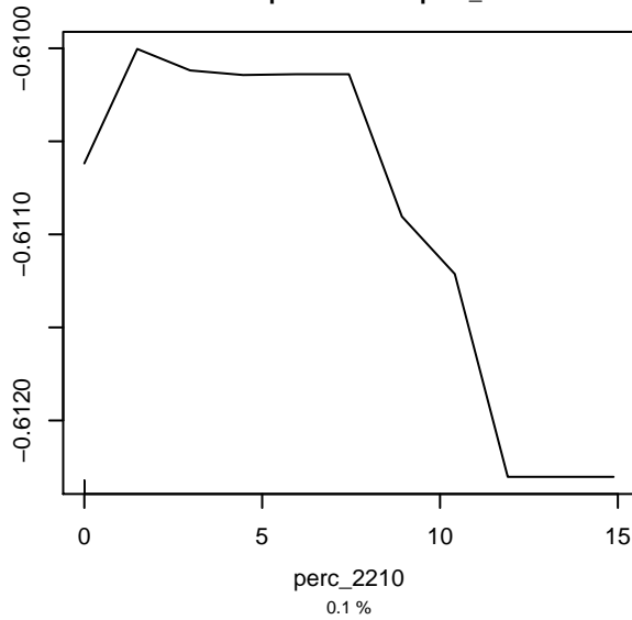
Partial dependence on perc_2210
