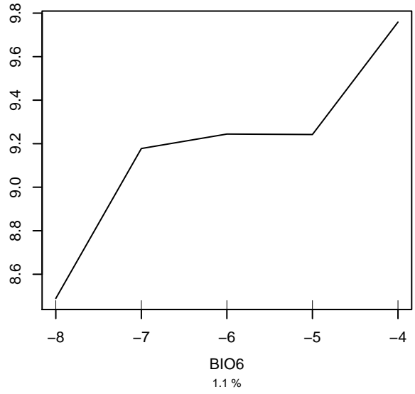
Partial dependence on BIO6
