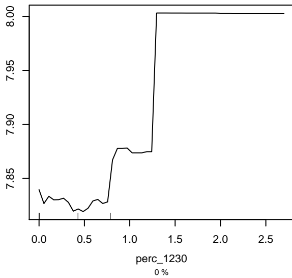
Partial dependence on perc_1230
