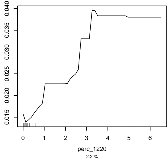
Partial dependence on perc_1220
